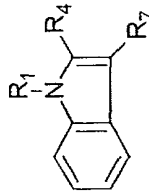
Ligand D IC_{50} = 1.2 \times 10^{-5} M
